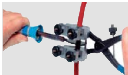
Welding paddle manual tool
